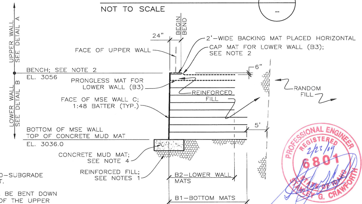
LOWER WALL STA. 0+00 TO 0+32 NOT TO SCALE
