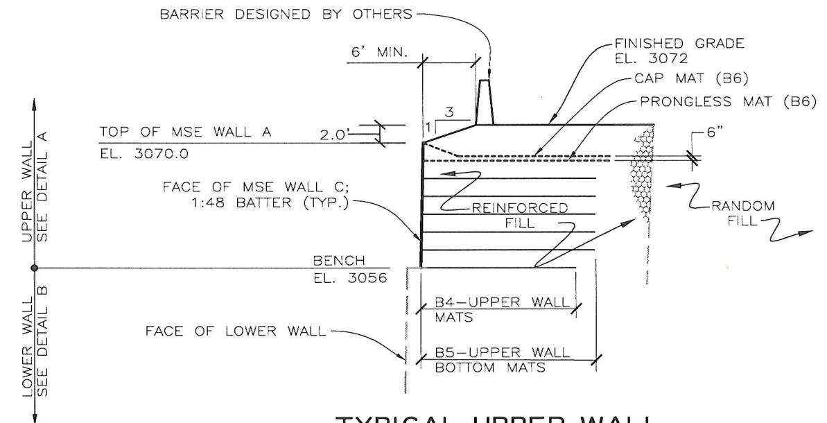
TYPICAL UPPER WALL STA. 0+00 TO 2+00 NOT TO SCALE
