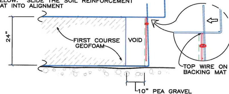
CONSTRUCTION SEQUENCE NOT TO SCALE
