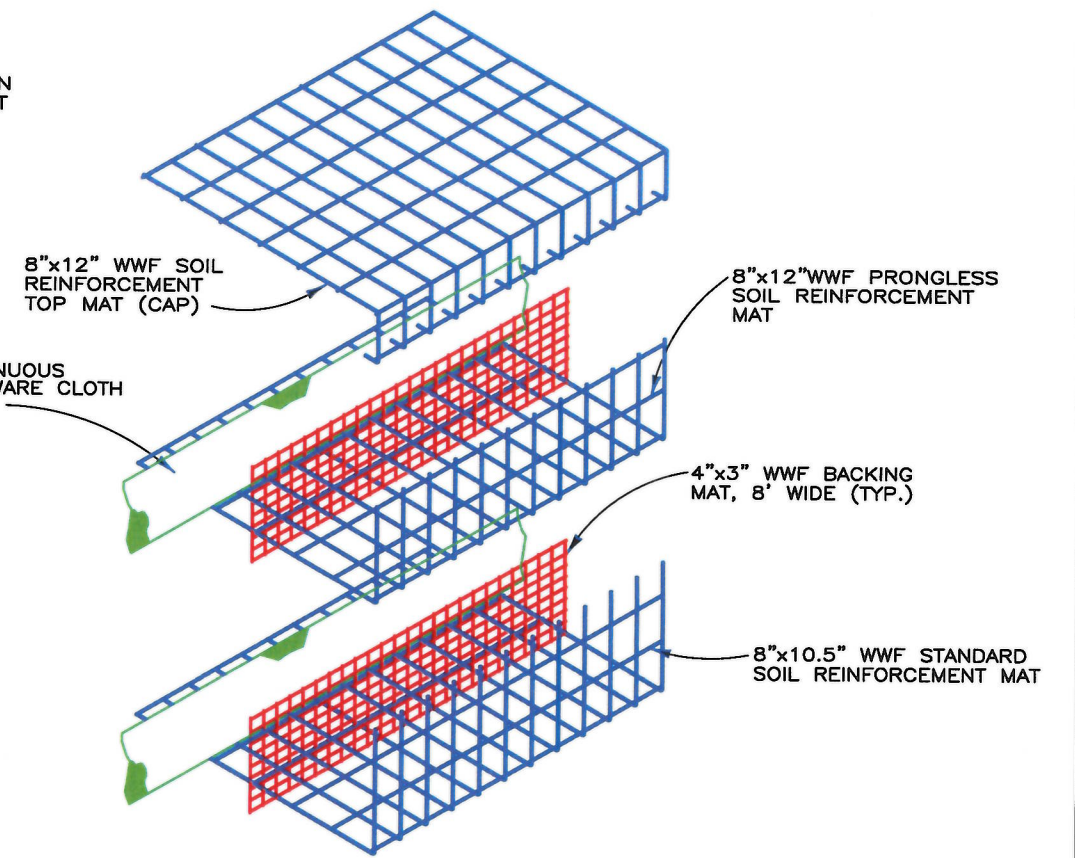
WELDED WIRE WALL COMPONENTS NOT TO SCALE
