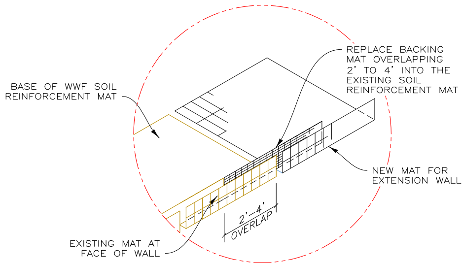
BACKING MAT REPLACEMENT NOT TO SCALE
