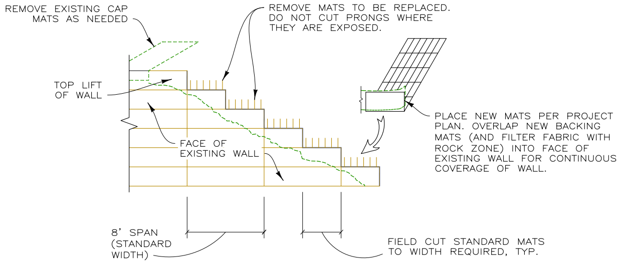
PICTORIAL ELEVATION CONNECTION TO EXISTING WALL SCALE: 1" = 10'
