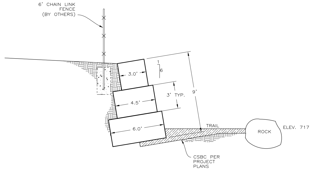
OPTION 2 - TYPICAL SECTION PER HRW STANDARD CONFIGURATION SCALE: 1" = 5'
