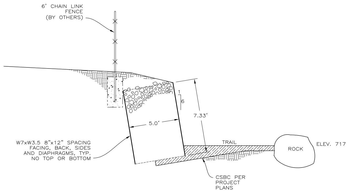
OPTION 3 - TYPICAL SECTION PER HRW STANDARD CONFIGURATION SCALE: 1" = 5'
