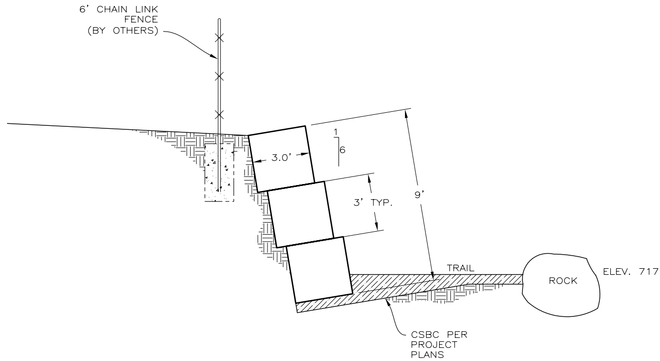
OPTION 1 - TYPICAL SECTION PER PROJECT PLANS SCALE: 1" = 5'
