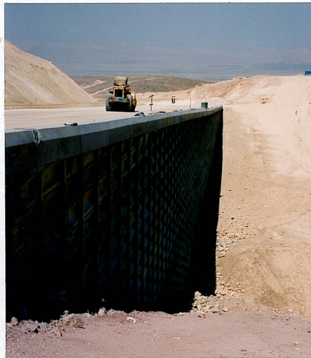
Dead Sea Highway Amman, Jordan Jordanian Ministry of Public Works Hudhud Shand Ltd. Summer 1990 Reinforced Soil Embankment
