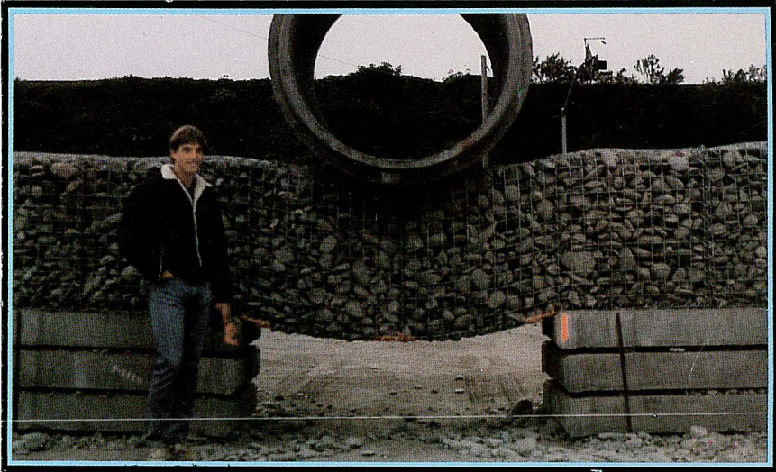
↑ ARTWELD GABION - EUREKA, CA. Strength Test for CALTRANS
